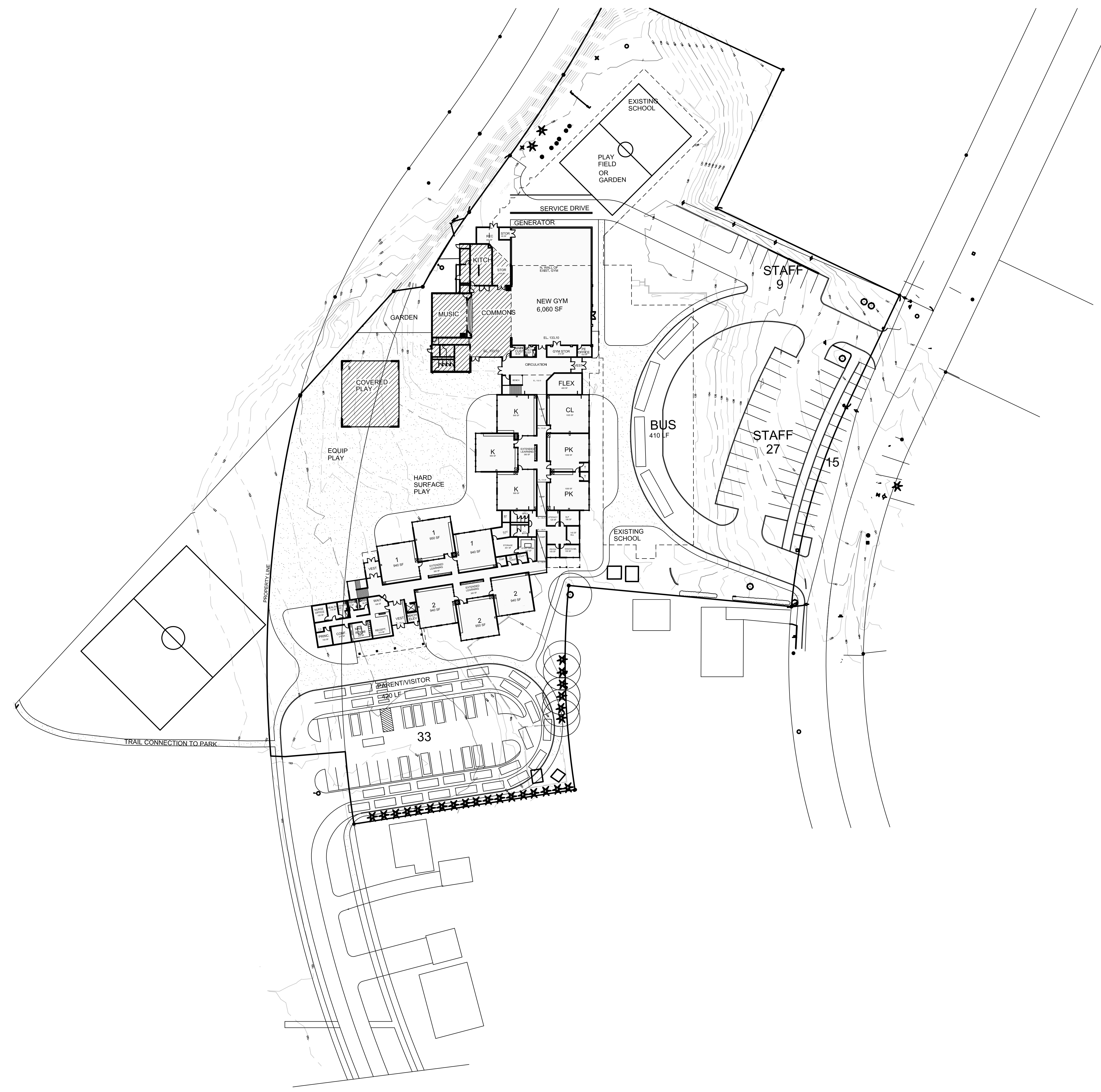
1 SITE PLAN 1" = 40'-0"
